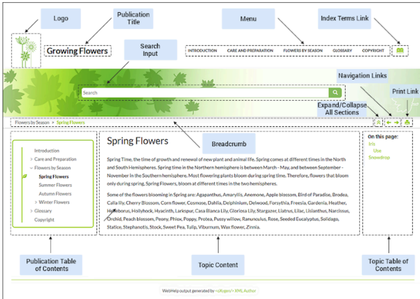
Figure 323. Topic Page
