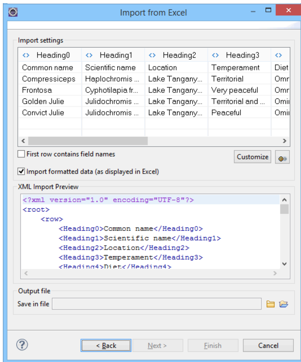
Figure 382. Import Wizard
