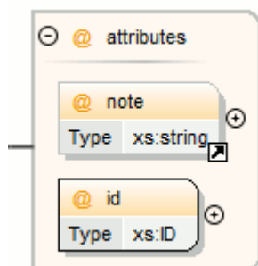
Figure 171. Attributes Construct
