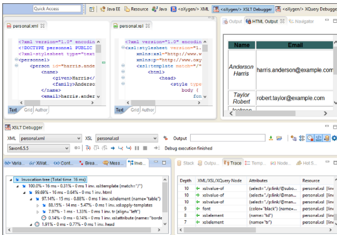
Figure 385. Debugger Interface
