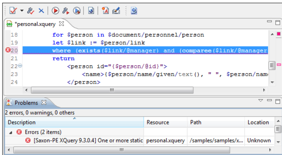
Figure 195. XQuery Validation
