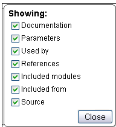
Figure 126. Showing Options
