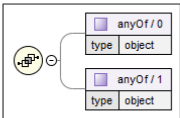
Figure 268. Example of an anyOf Component
