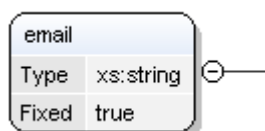
Figure 147. The xs:element Component
