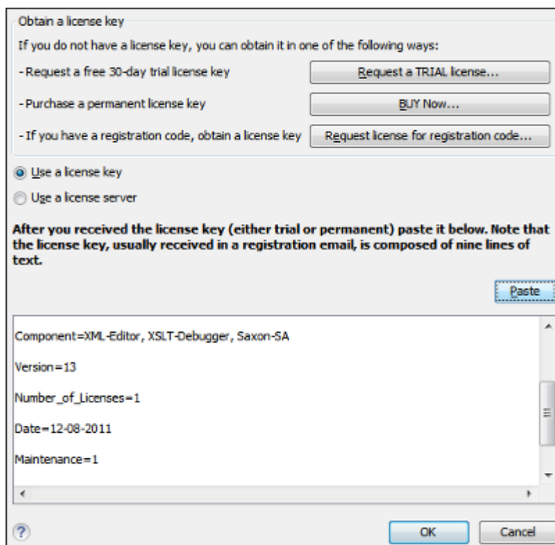
Figure 2. License Registration Dialog Box
