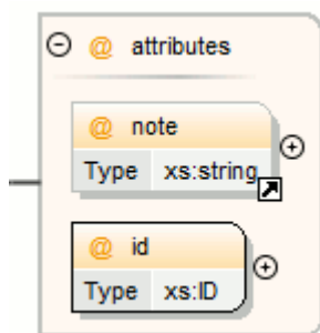
Figure 329. Attributes Construct
