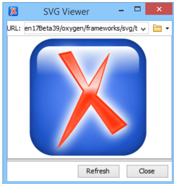
Figure 464. SVG Viewer
