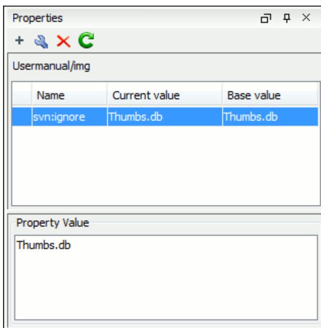
Figure 753. Properties View
