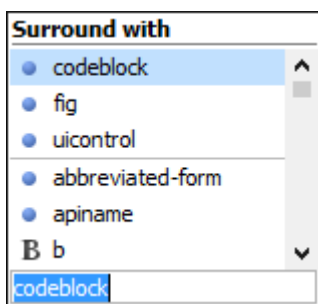
Figure 154. Example (Surround)
