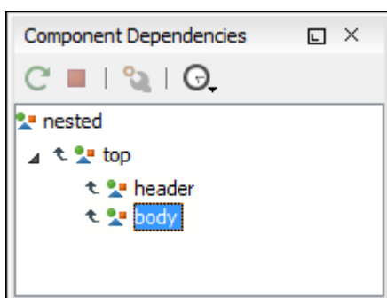
Figure 392. Component Dependencies View
