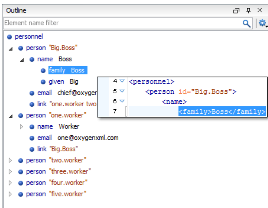
Figure 157. Outline View
