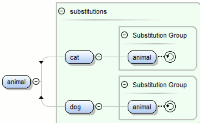
Figure 331. Substitutions Construct
