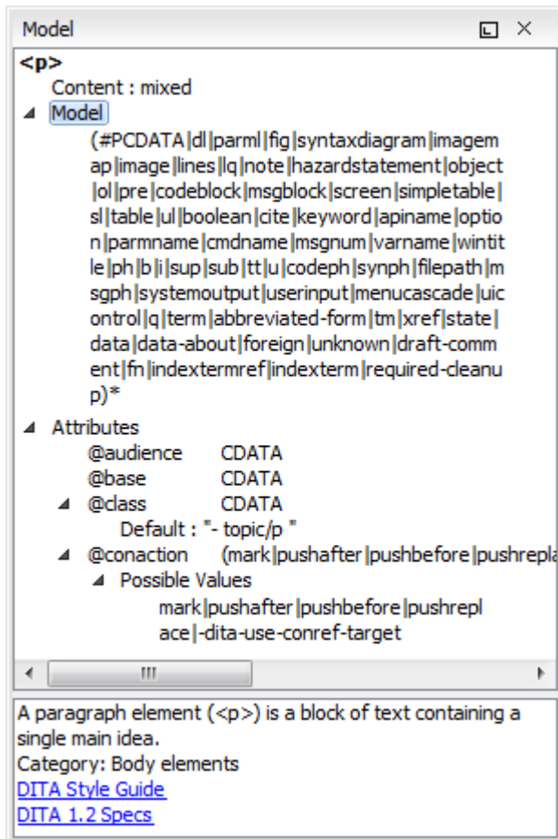
Figure 161. Model View
