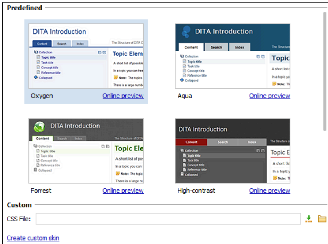
Figure 485. Skins Tab
