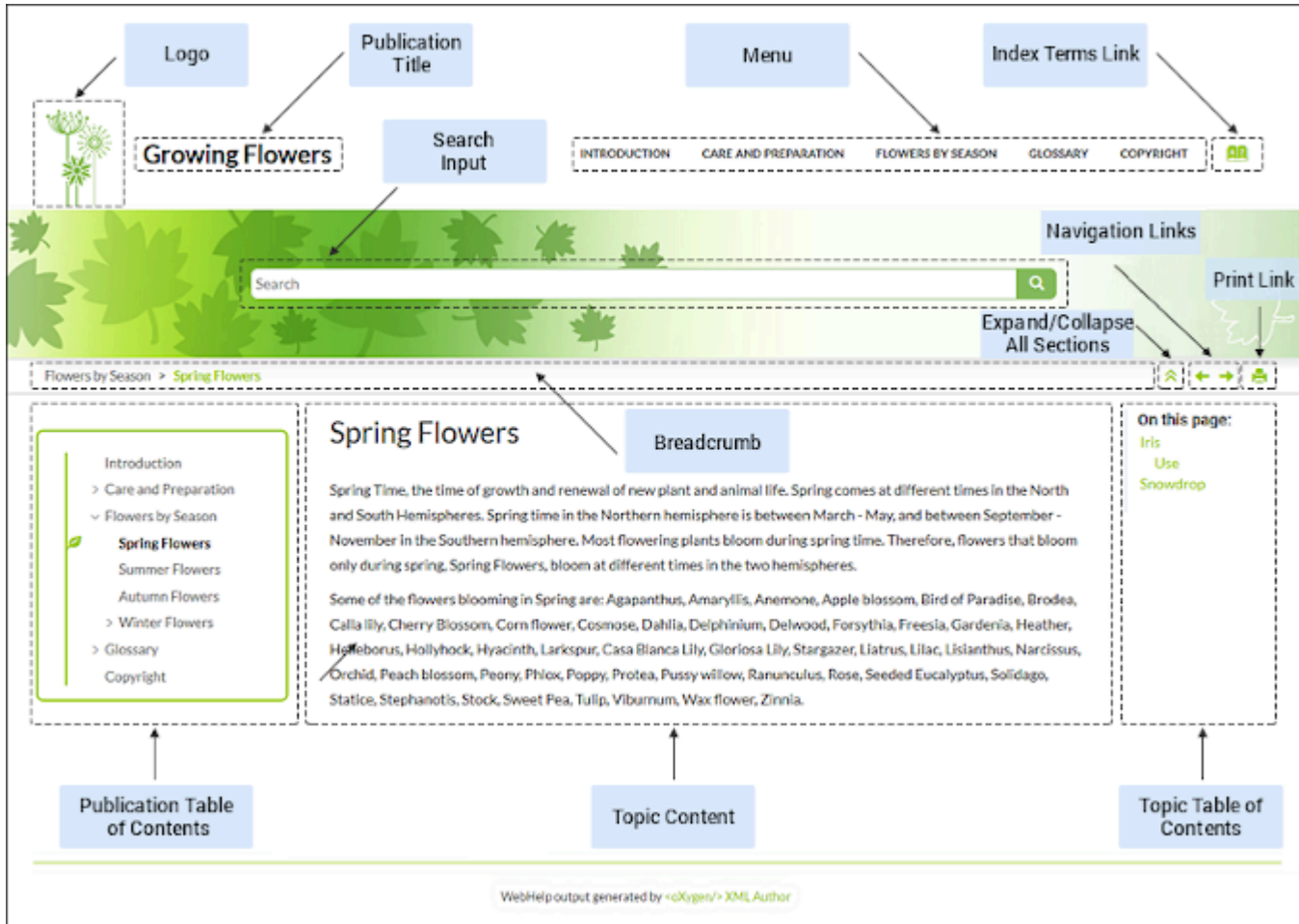
Figure 500. Topic Page
