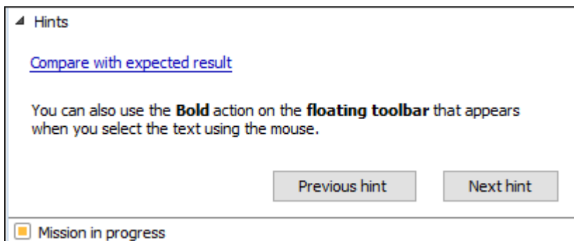
Figure 630. Hints Pane
