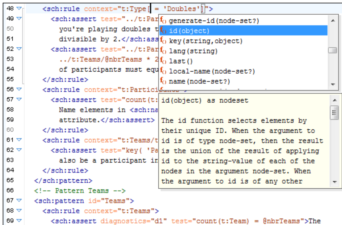
Figure 455. XSLT Extension Functions in Schematron Schema Content Completion
