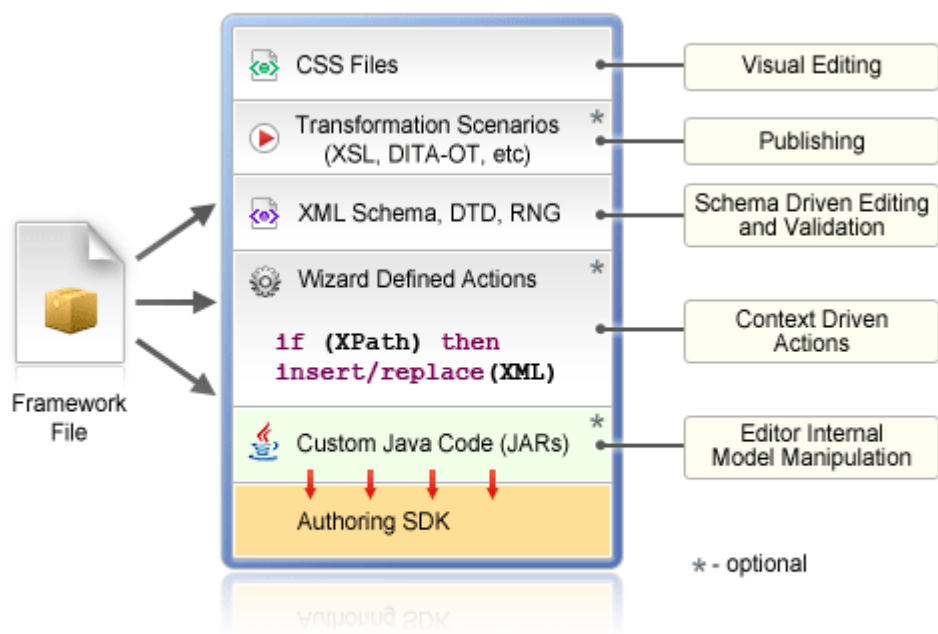
Figure 621. Components of a Custom Framework
