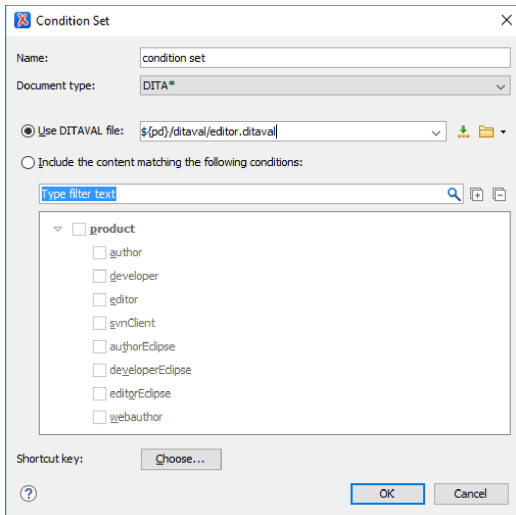
Figure 828. Condition Set Configuration Dialog Box
