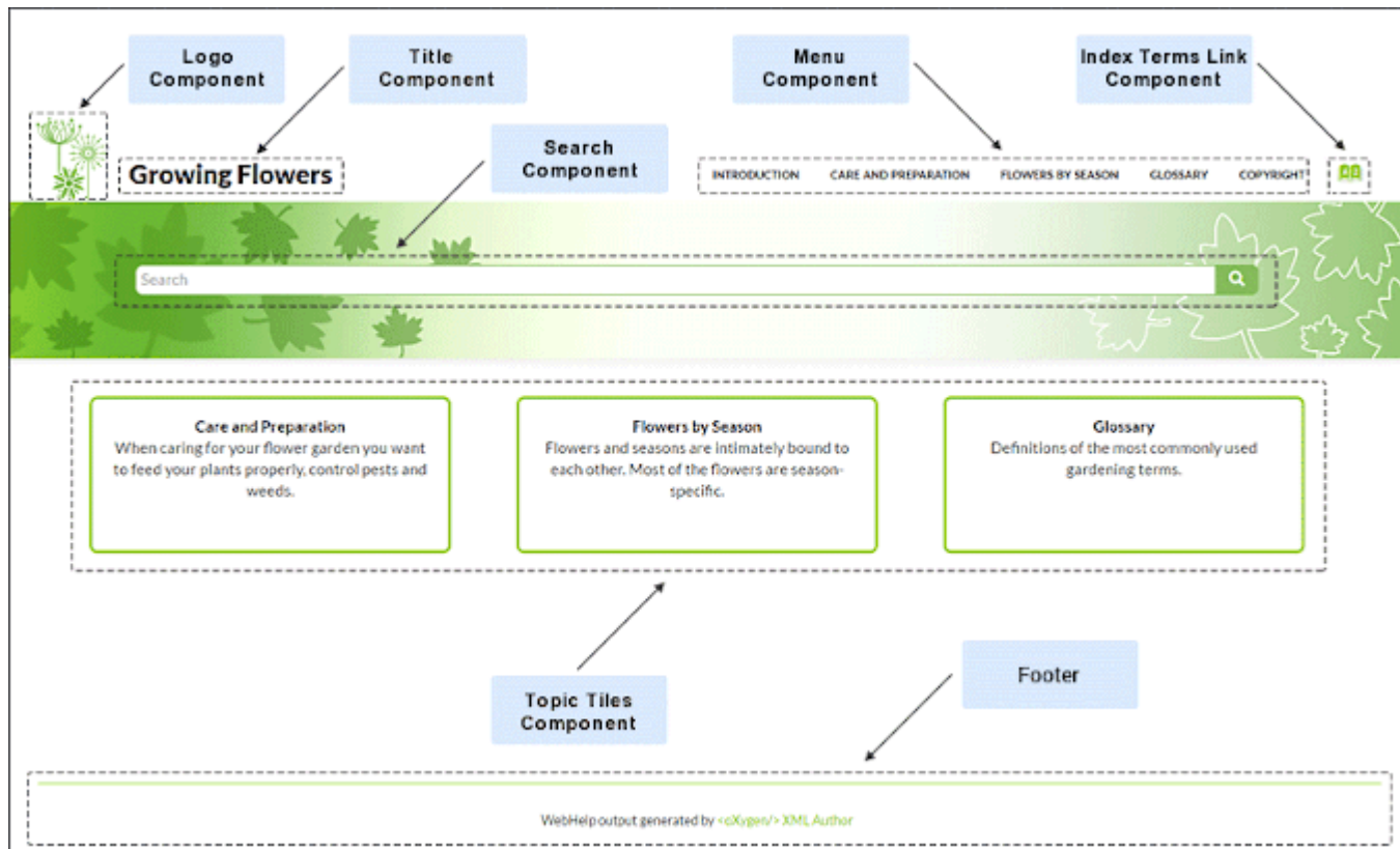
Figure 498. Main Page - Tiles Layout
