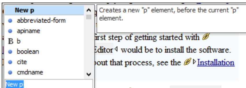
Figure 155. Schema Annotation in the Content Completion Assistant
