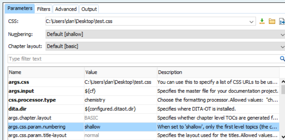
Figure 837. Promoted Parameters
