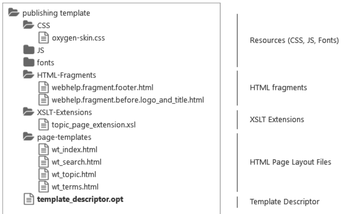
Figure 294. Oxygen Publishing Template Package (WebHelp Responsive)
