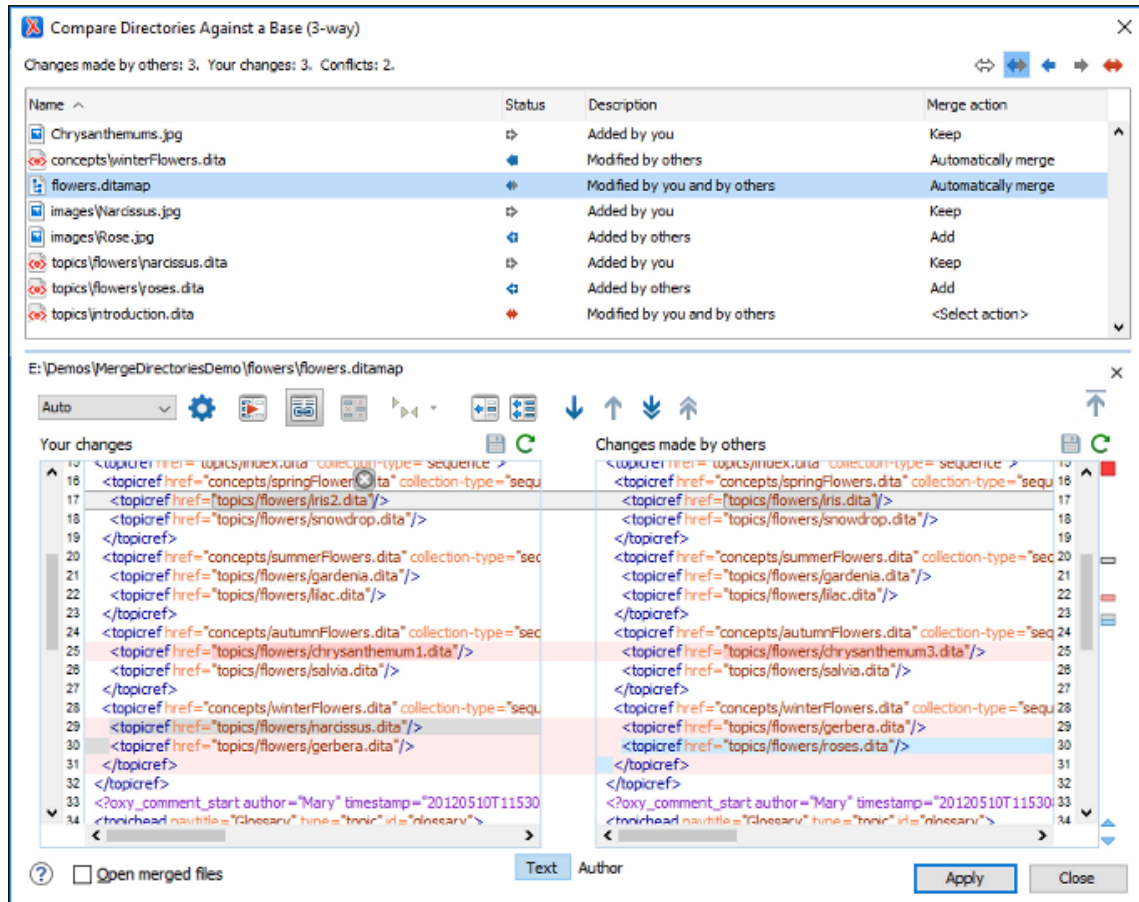
Figure 415. Comparison and Merge Tool
