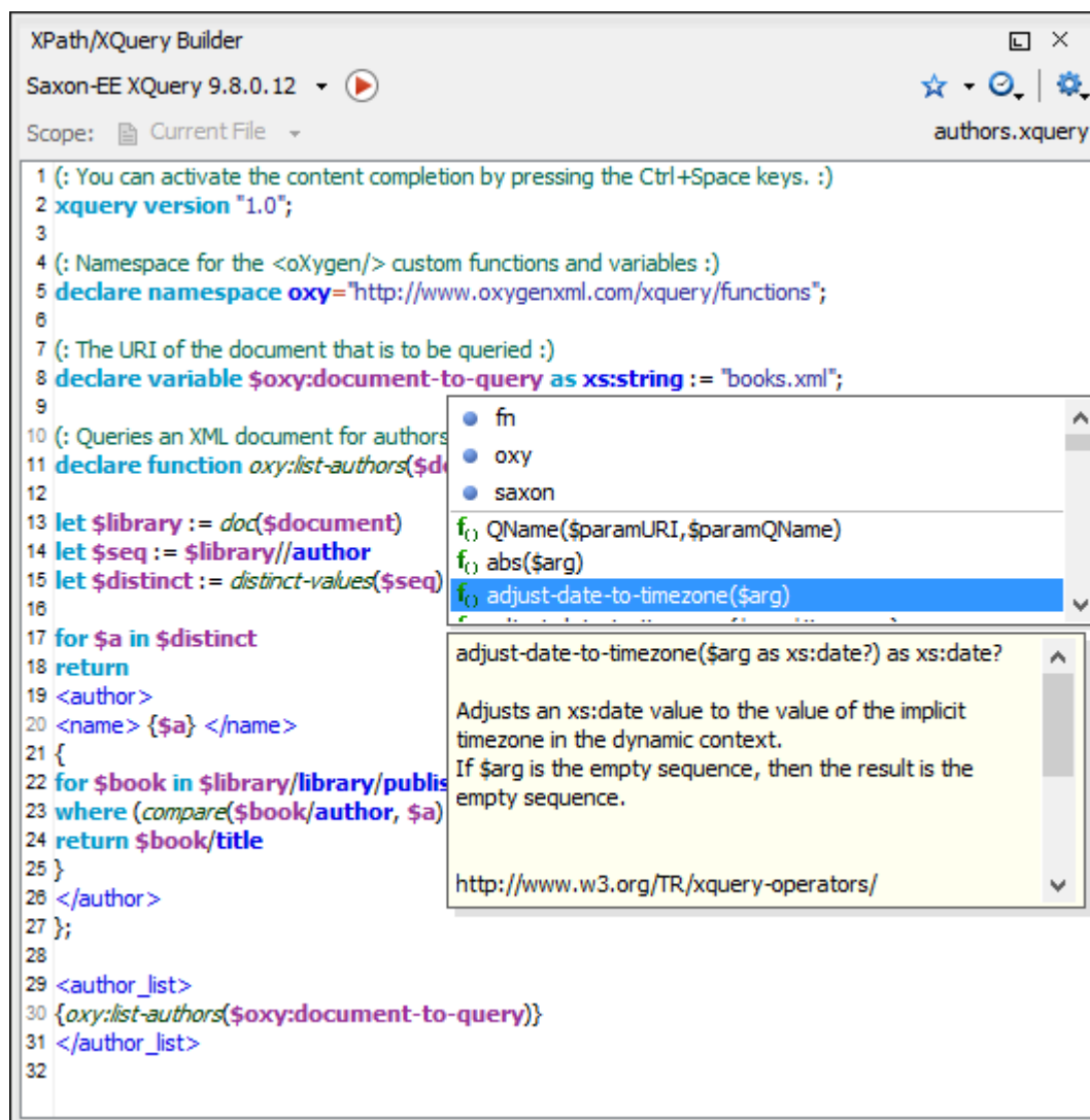
Figure 320. XPath/XQuery Builder View
