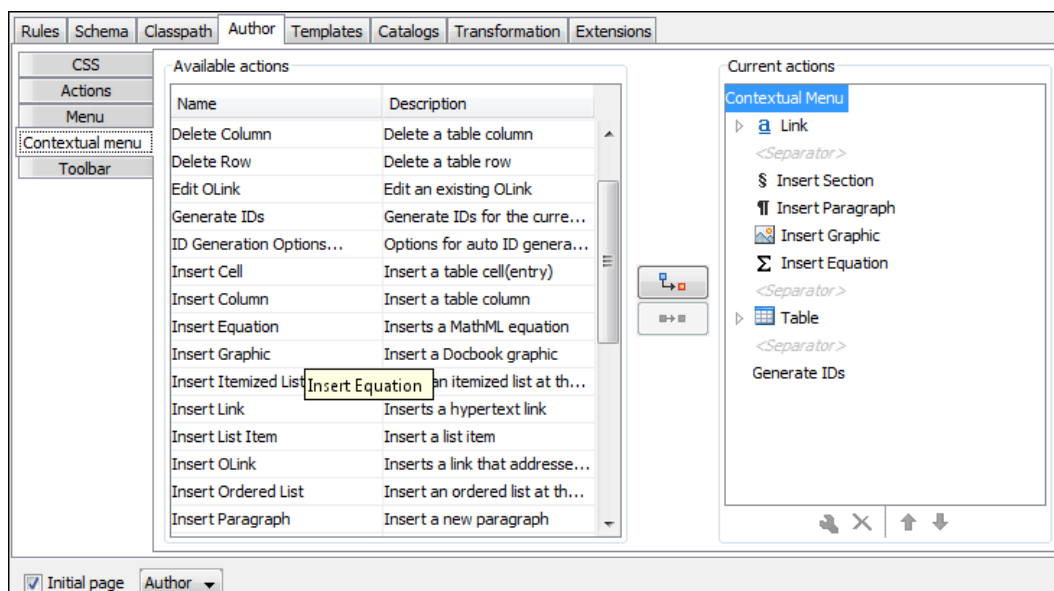
Figure 356. Configuring the Contextual Menu
