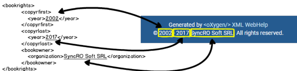
Figure 307. Example: Copyright Information Added in the WebHelp Footer
