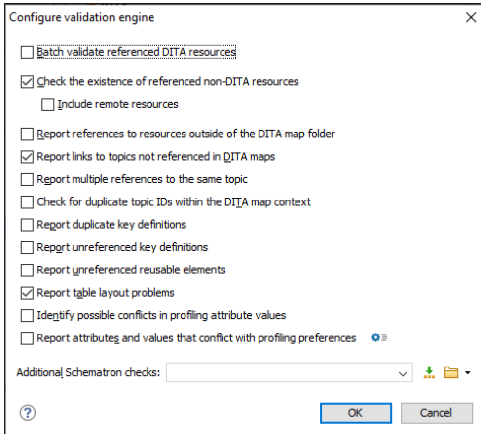
Figure 555. Configure Validation Engine Dialog Box for DITA-OT Project Validation
