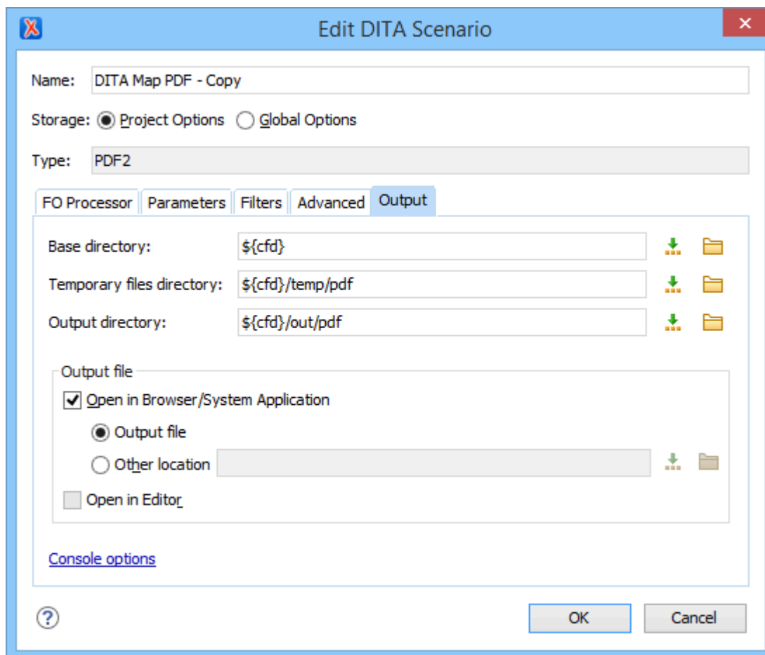
Figure 540. Output Settings Tab
