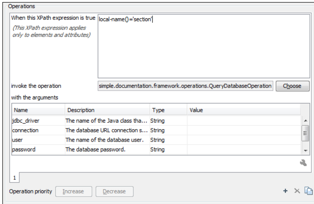
Figure 378. Java Operation Arguments Setup
