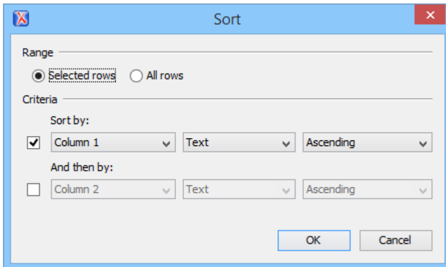
Figure 208. Sort Selected Rows
