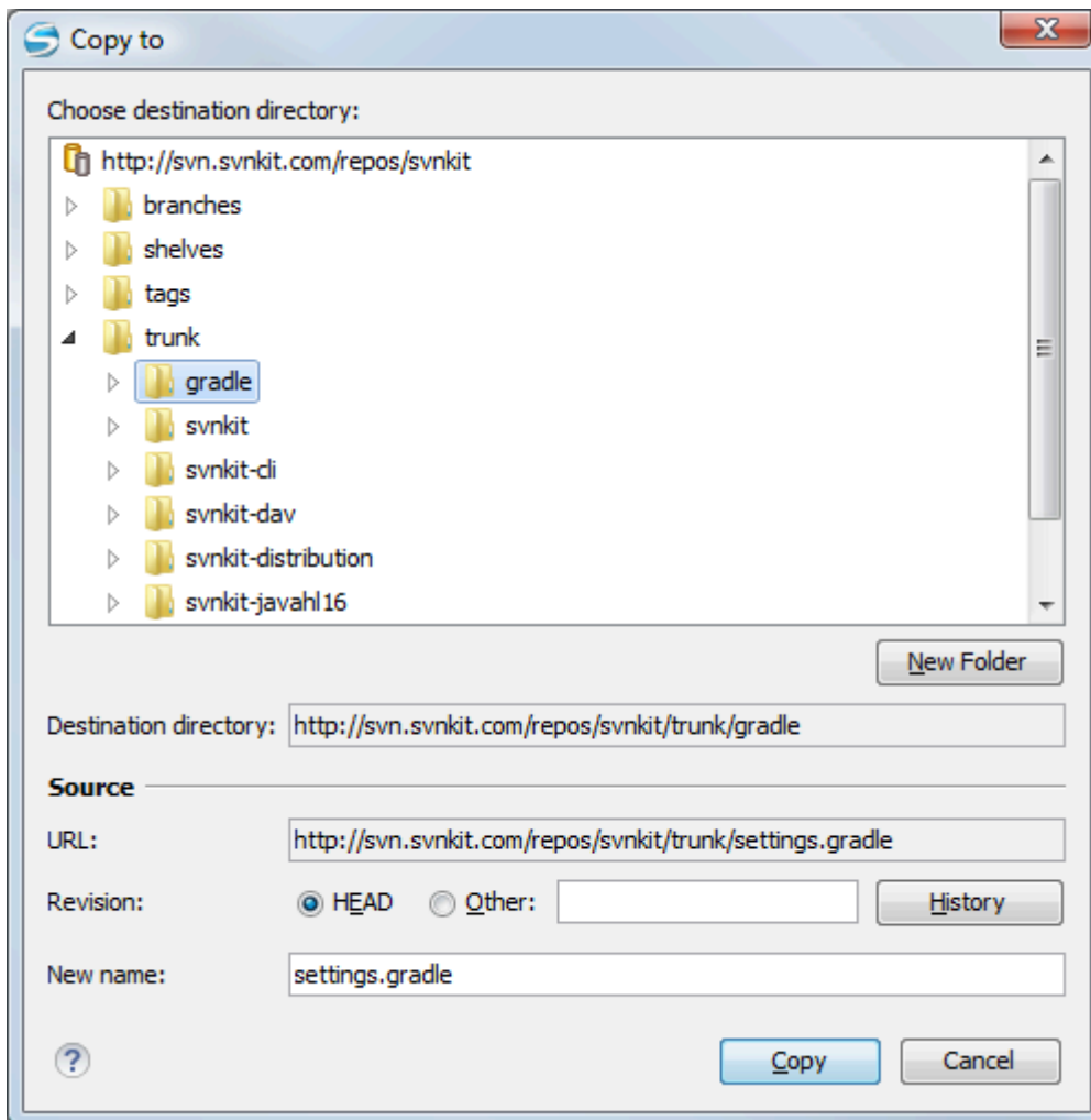
Figure 455. Copy/Move Items in Repository
