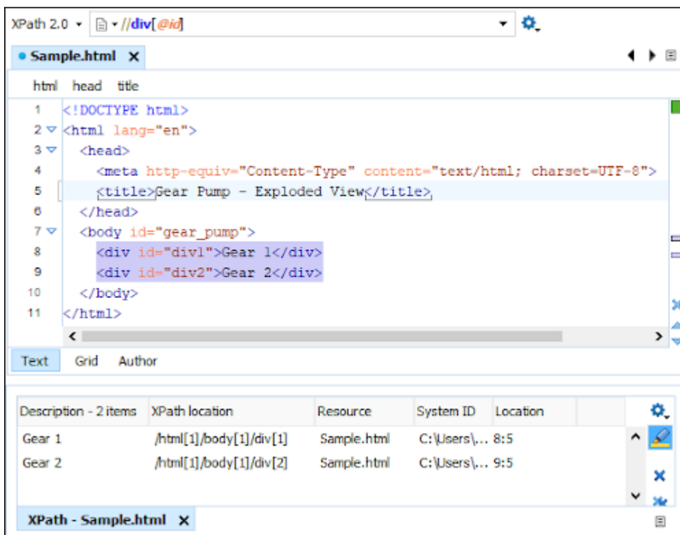
Figure 260. XPath Toolbar for HTML
