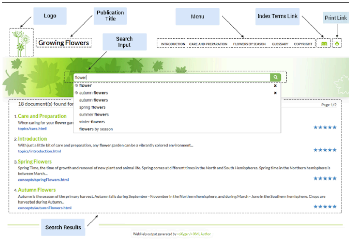
Figure 301. Examples of Search Results Page Components
