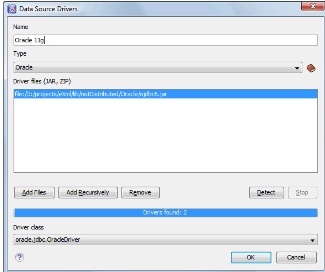
Figure 331. Data Source Drivers Configuration Dialog Box
