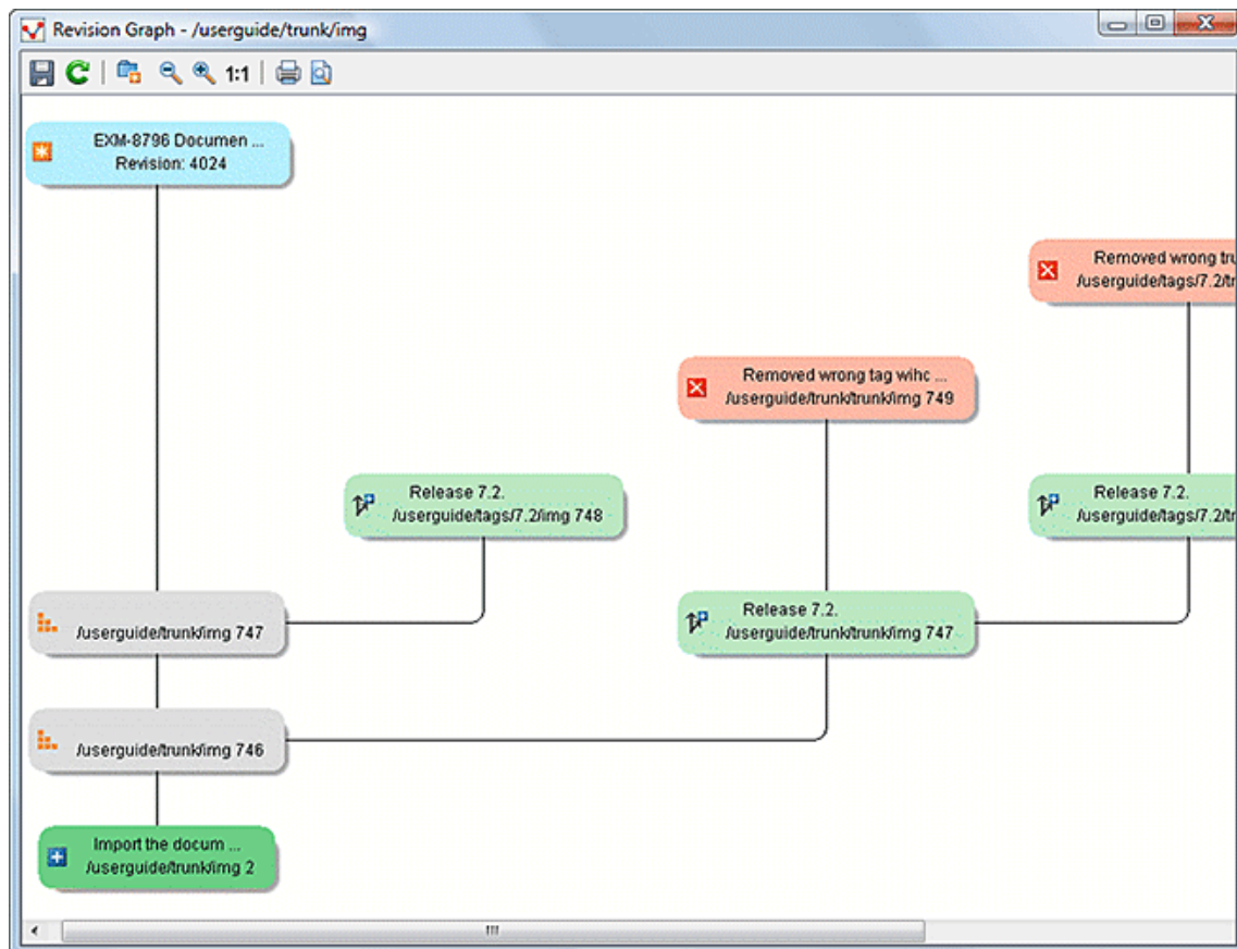
Figure 472. Revision Graph of a Directory (Direct Changes)
