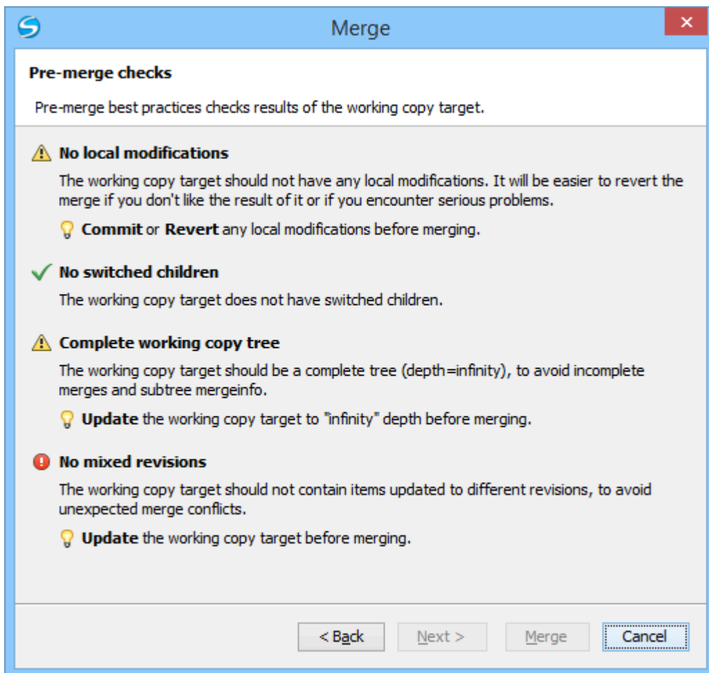
Figure 440. Pre-Merge Checks Wizard Page
