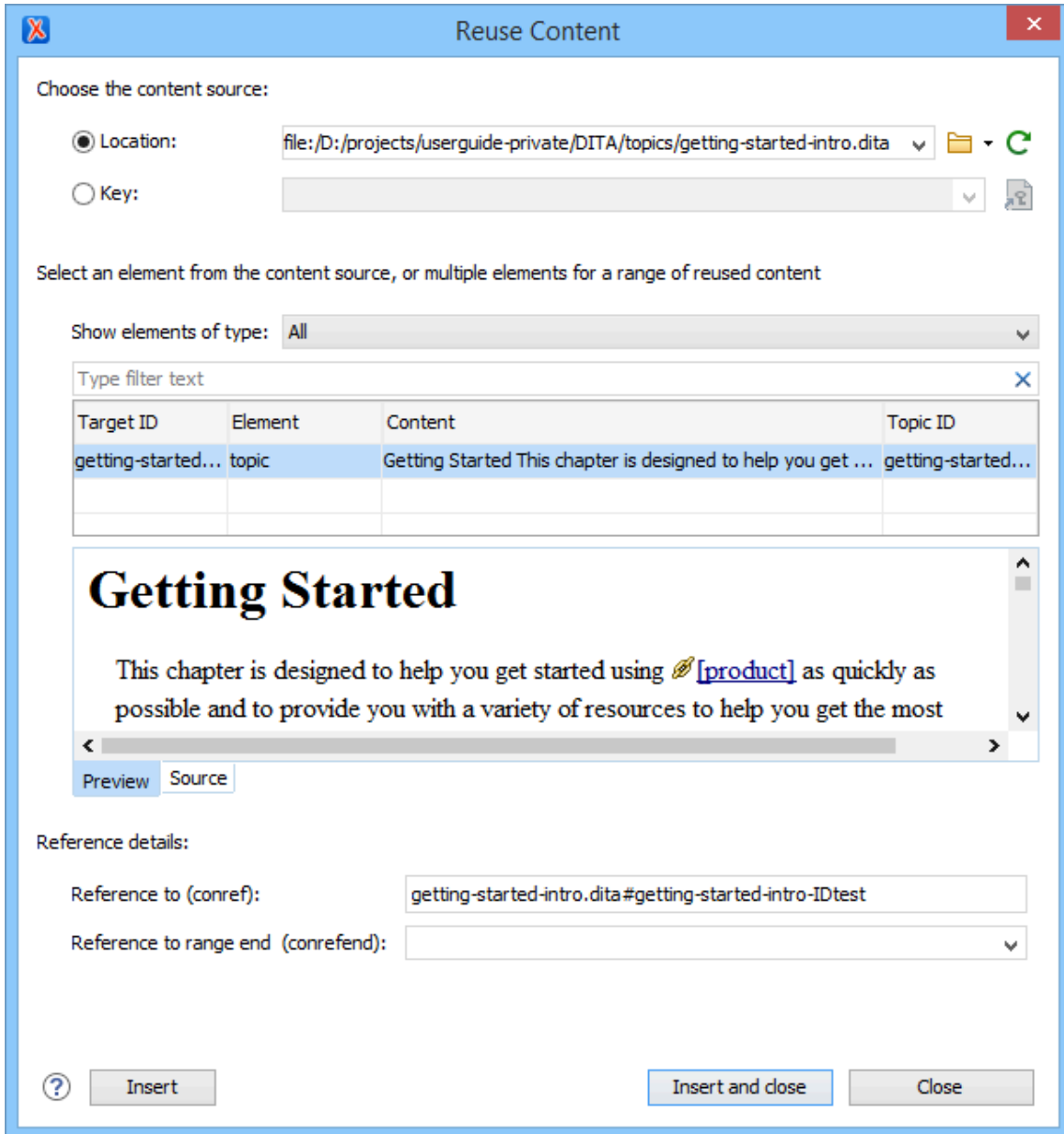
Figure 518. Reuse Content Dialog Box (with the Default Insert Content Reference Options Displayed)
