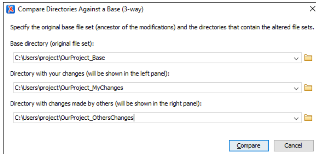
Figure 414. Compare Directories Against a Base File Set Chooser
