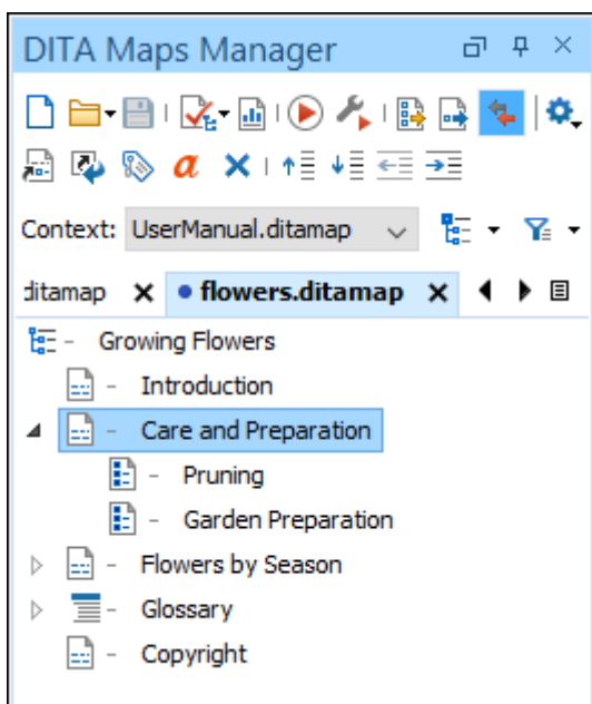
Figure 479. DITA Maps Manager View
