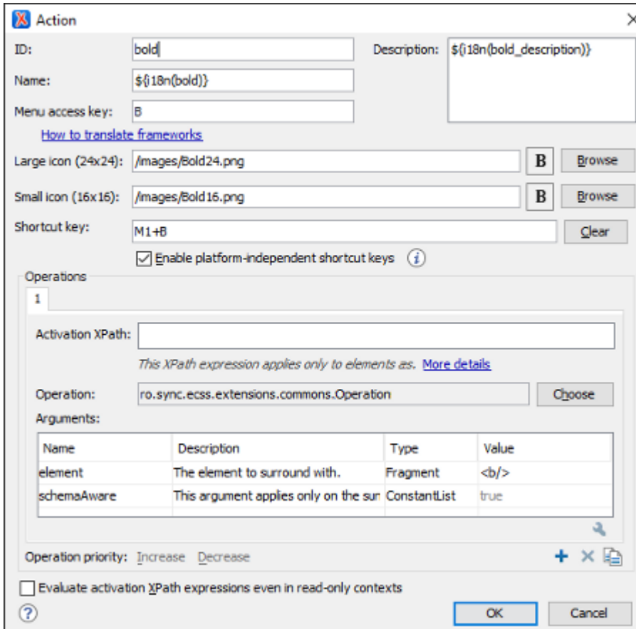
Figure 23. Action Dialog Box
