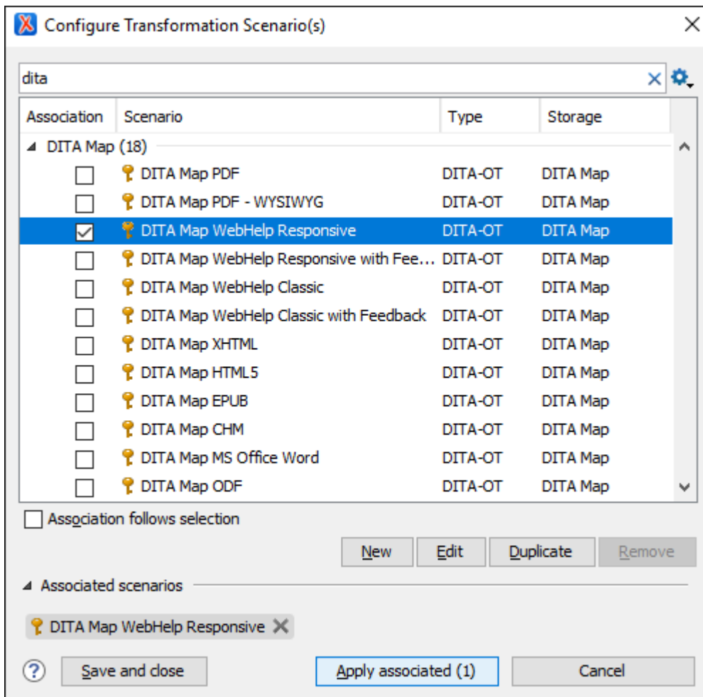
Figure 478. Configure Transformation Scenarios Dialog Box
