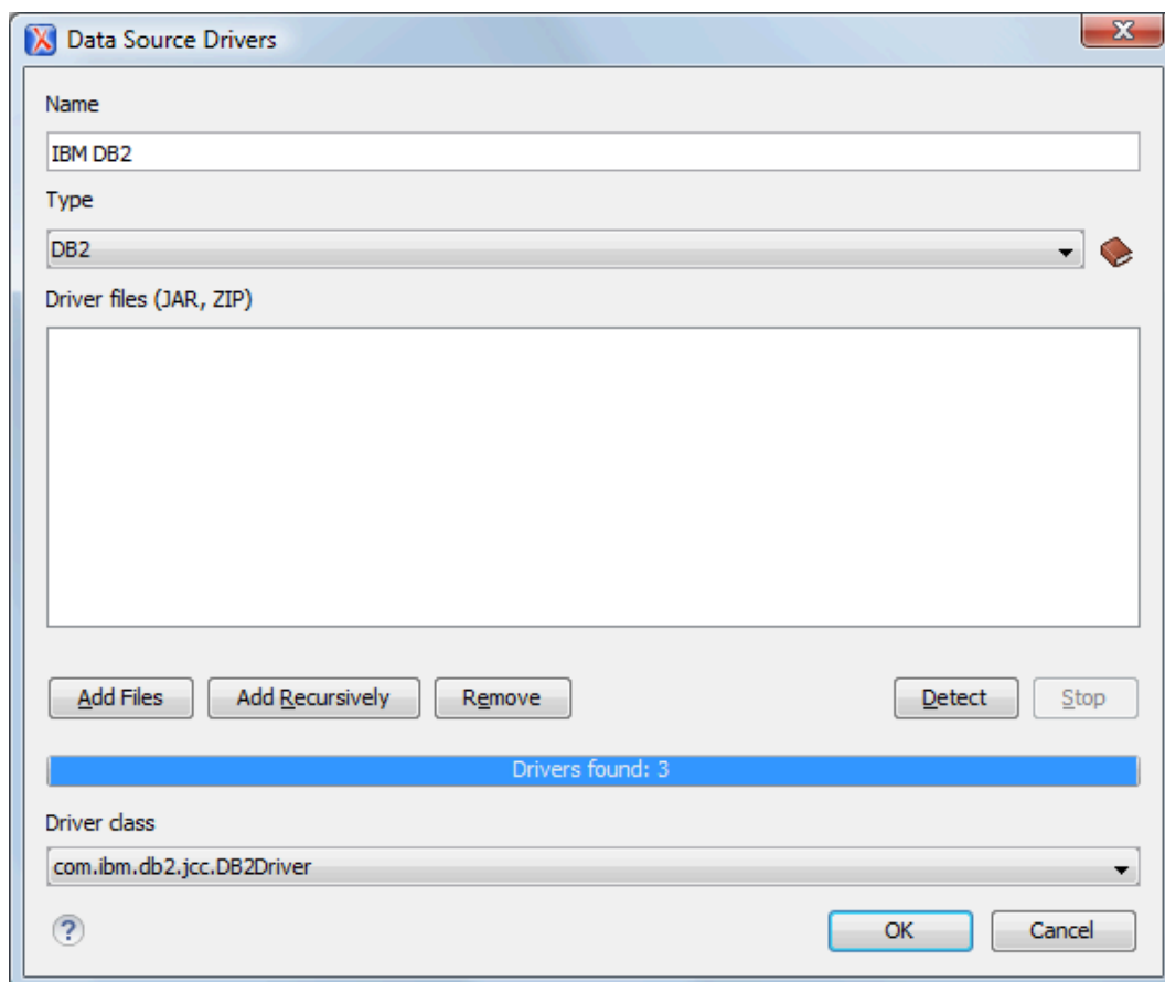
Figure 341. Data Source Drivers Configuration Dialog Box
