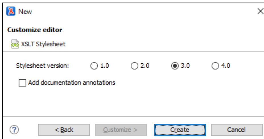
Figure 59. New XSLT Stylesheet Configuration Wizard Page
