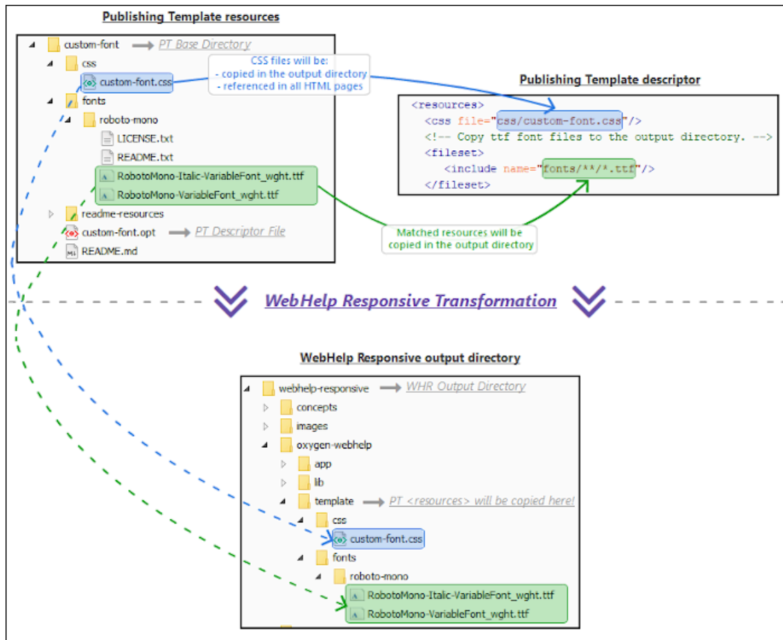
Figure 311. Referencing Local Fonts in a Publishing Template
