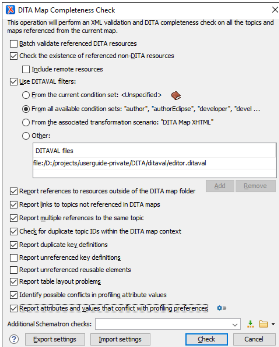
Figure 752. DITA Map Completeness Check Dialog Box
