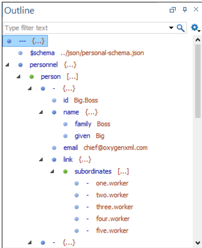
Figure 447. YAML Outline View
