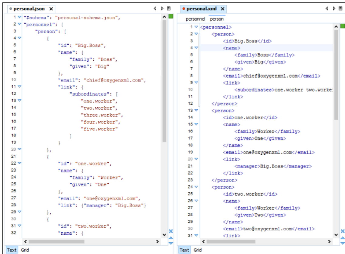
Figure 405. Example: XML to JSON Operation Result
