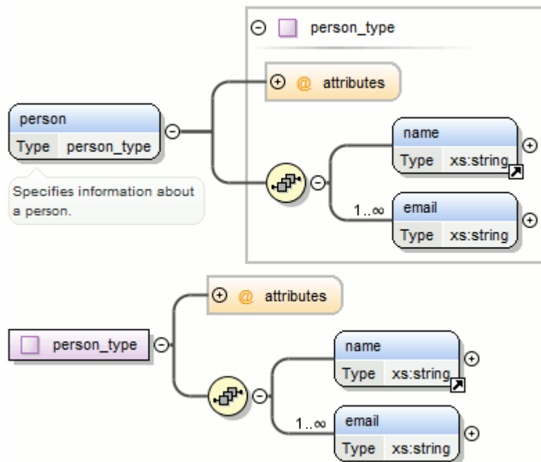
Figure 303. Extracting a Global Complex Type on a <person> Element
