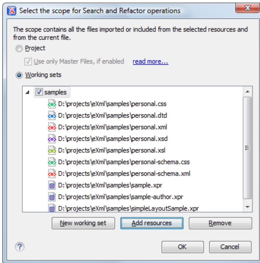
Figure 247. Change Scope Dialog Box
