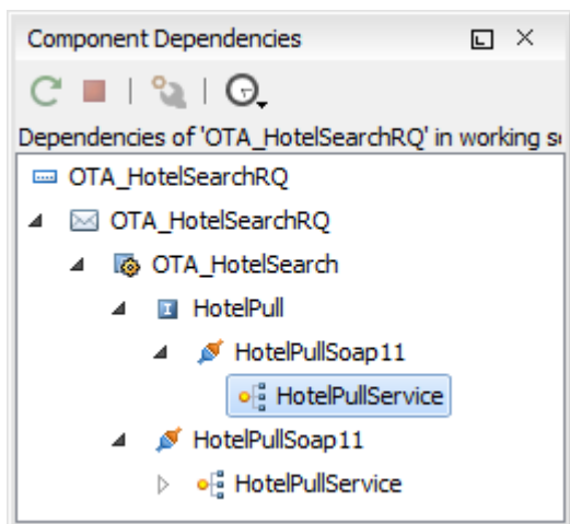
Figure 369. Component Dependencies View
