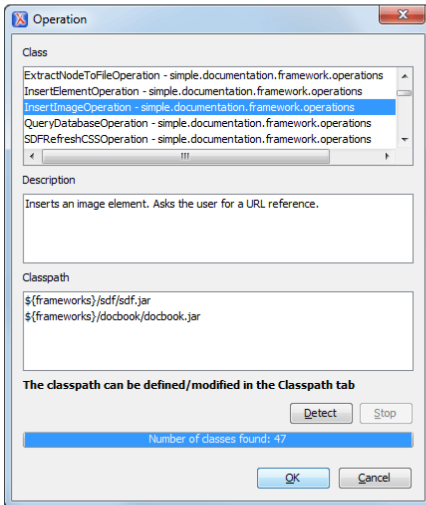
Figure 606. Selecting the Operation
