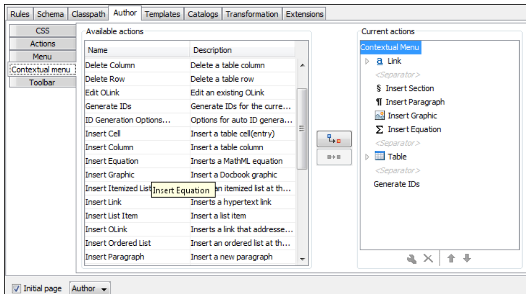
Figure 585. Configuring the Contextual Menu
