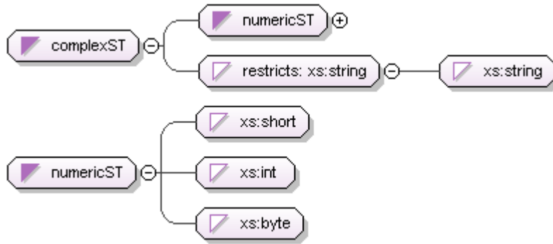
Figure 301. Extracting a Global Simple Type on a union Component
