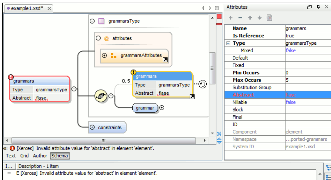
Figure 334. XML Schema Validation
