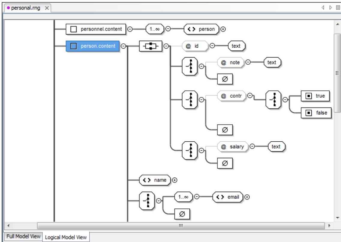
Figure 383. Logical Model View for a Relax NG Schema
