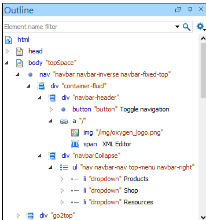
Figure 466. HTML Outline View
