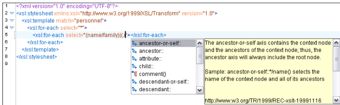
Figure 266. Content Completion in the @select Attribute
