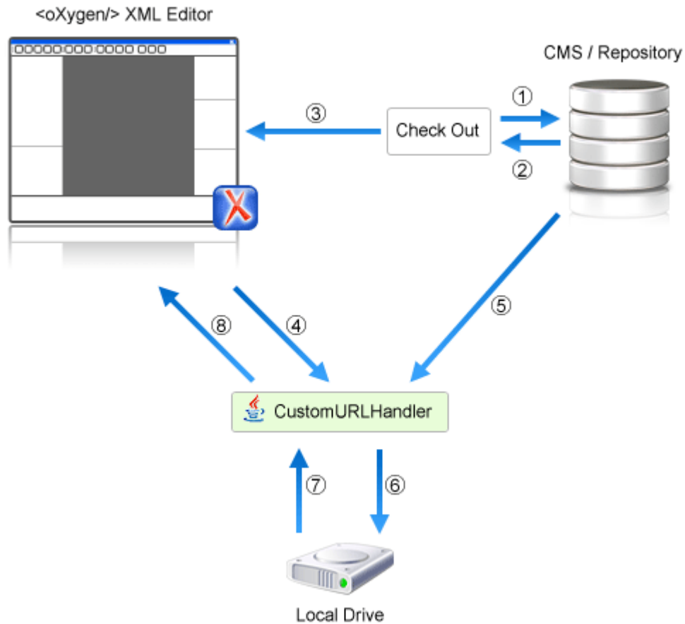
Figure 616. Check Out Process Diagram
