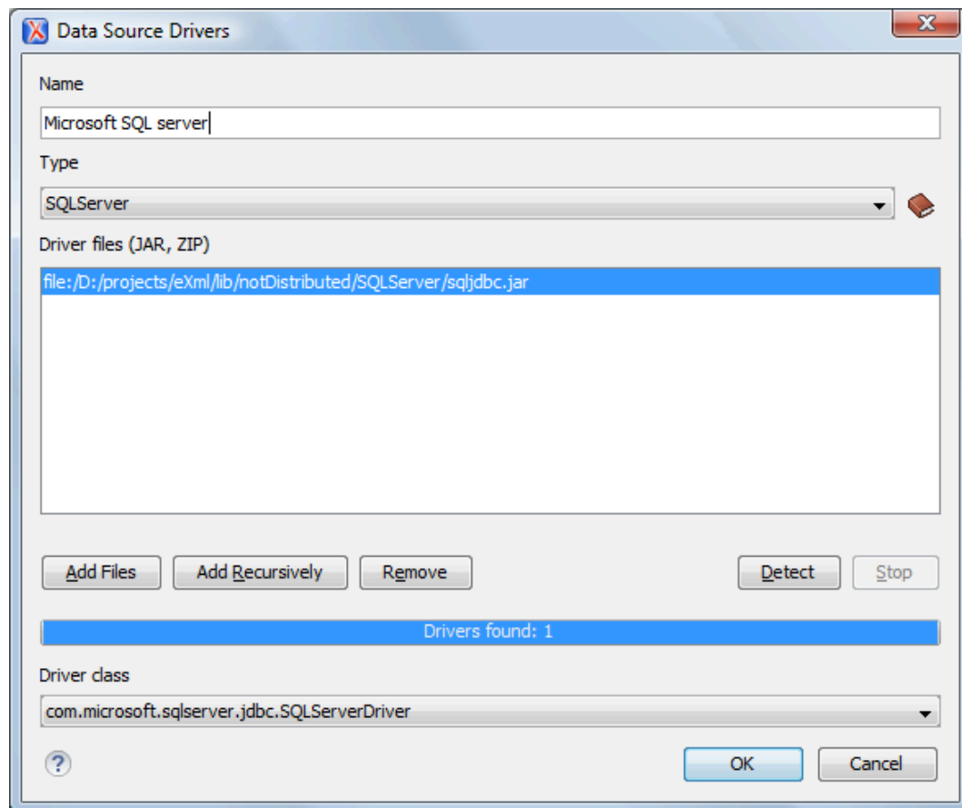
Figure 535. Data Source Drivers Configuration Dialog Box
