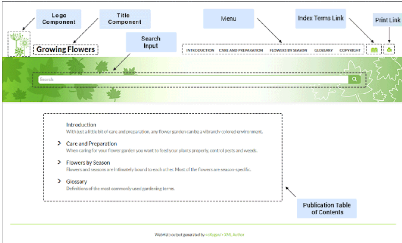
Figure 506. Examples of Main Page Components for a Tree Style of Layout
