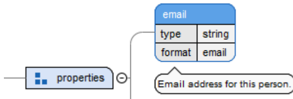
Figure 418. Example: Optional Component
