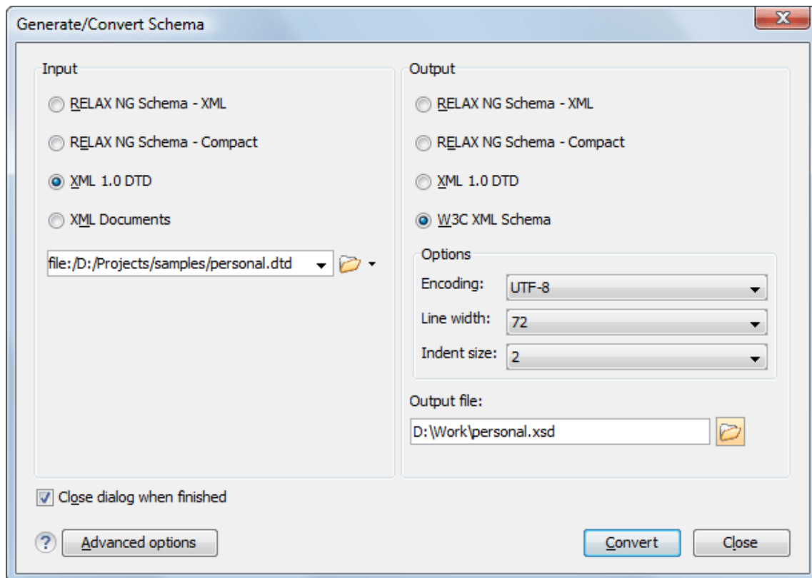
Figure 630. Generate/Convert Schema Dialog Box
