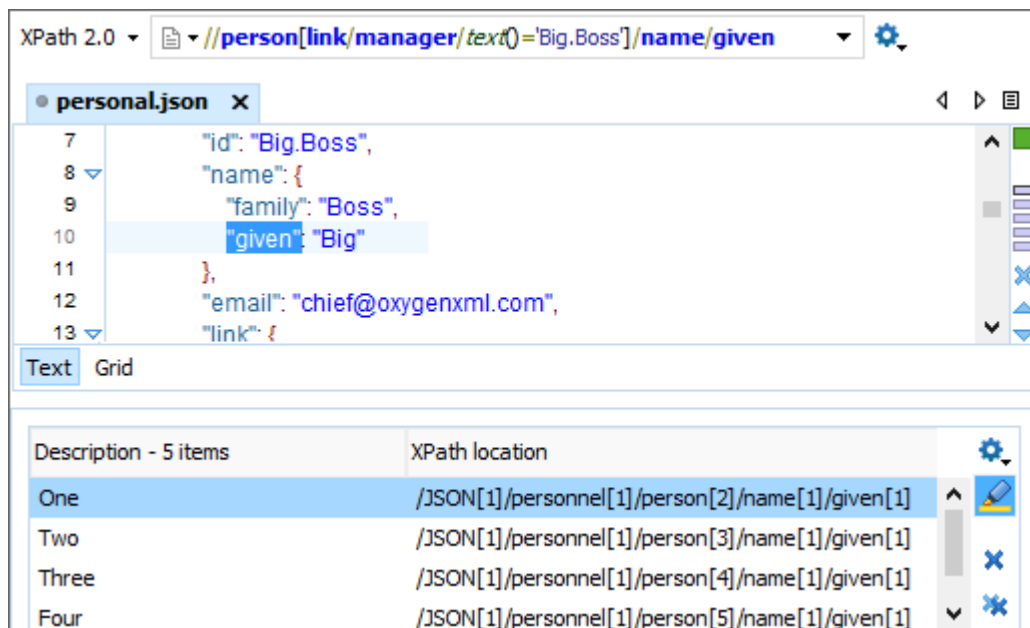
Figure 410. XPath Toolbar for JSON
