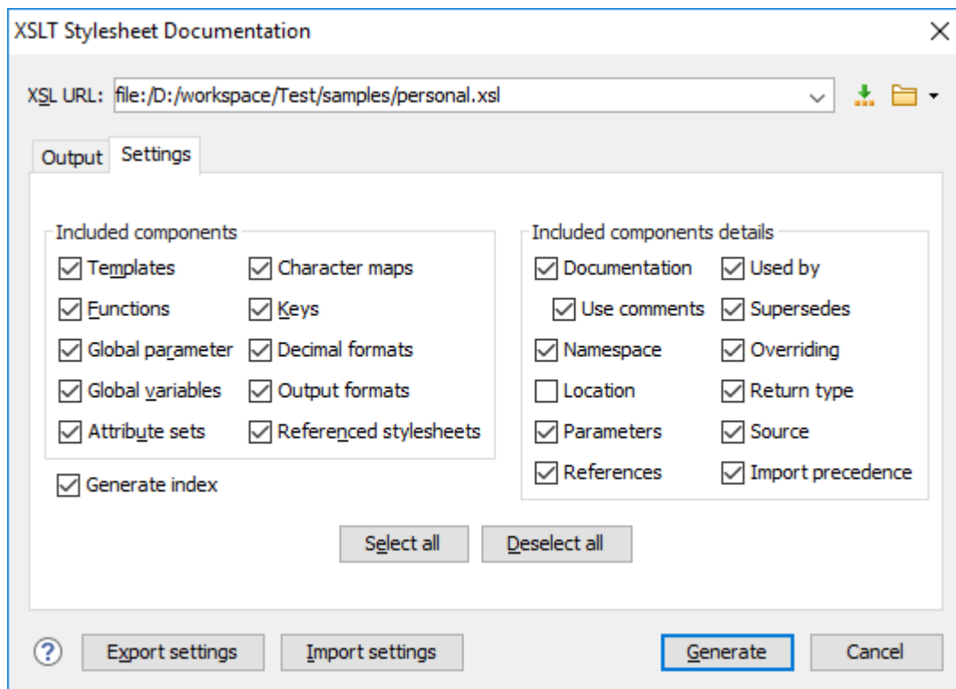
Figure 282. Settings Tab of the XSLT Stylesheet Documentation Dialog Box
