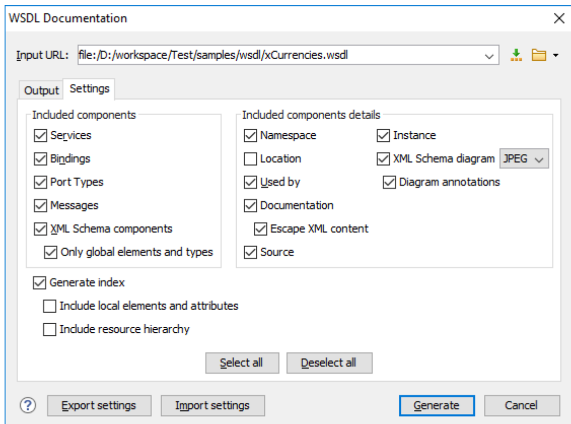
Figure 374. Settings Tab of the WSDL Documentation Dialog Box
