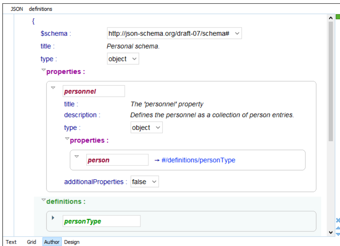
Figure 413. JSON Schema in Author Mode
