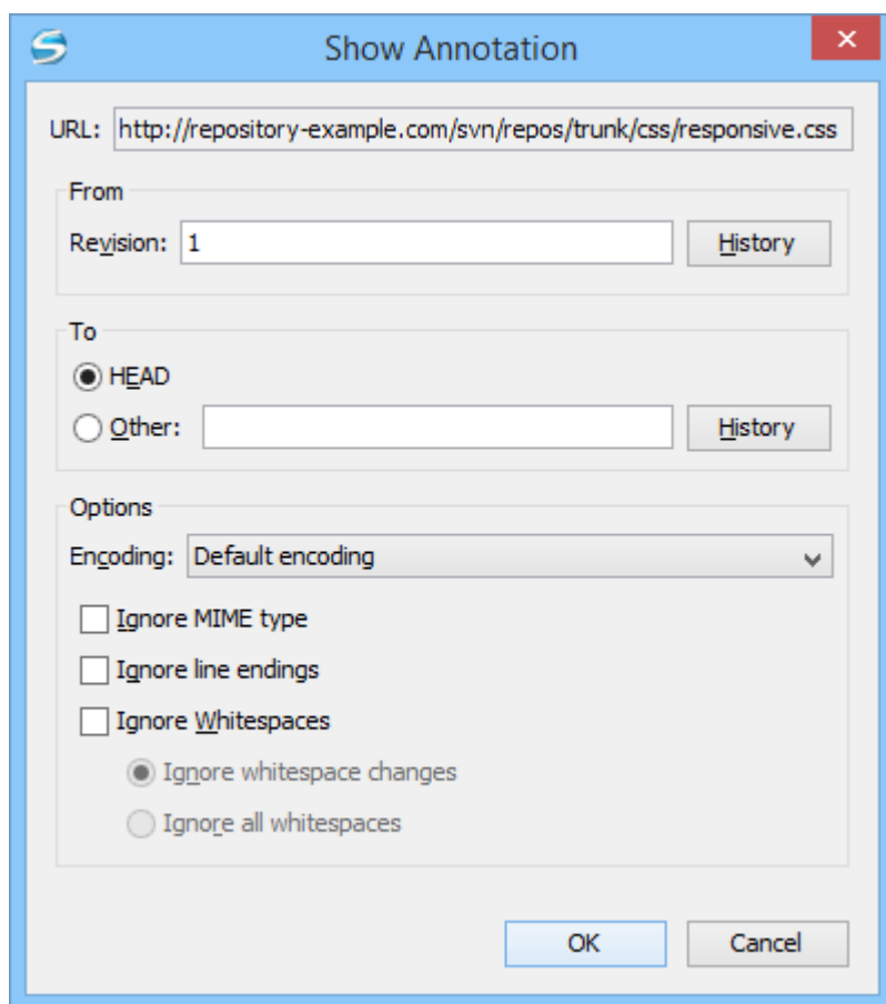
Figure 723. Show Annotation Options Dialog Box
