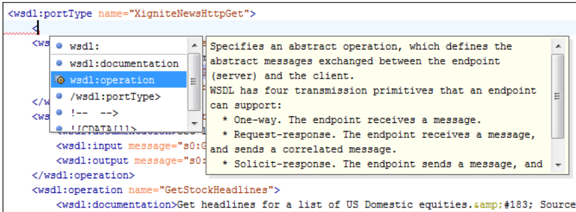
Figure 365. WSDL Content Completion Assistant
