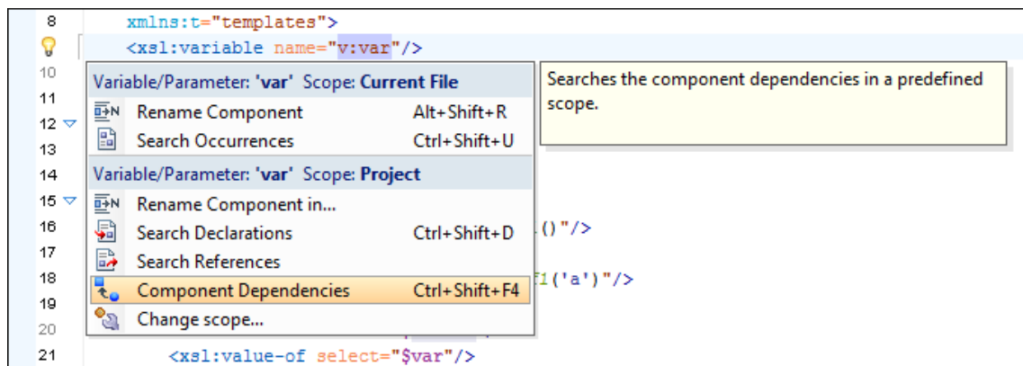
Figure 279. XSLT Quick Assist Support - Component Actions
