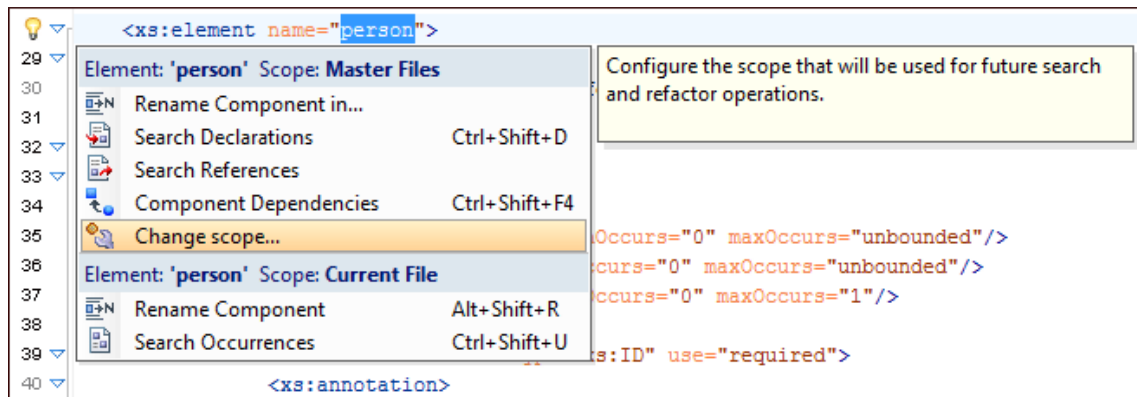
Figure 340. Quick Assist Support
