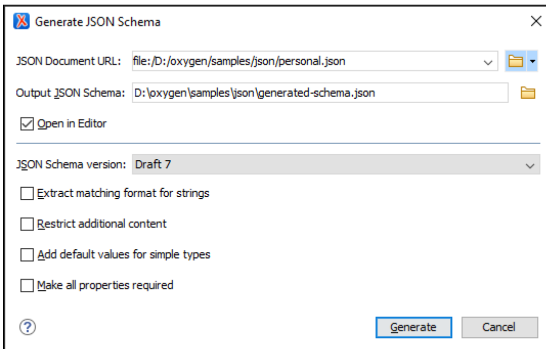
Figure 441. Generate JSON Schema Dialog Box
