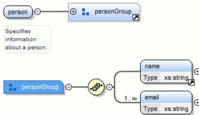
Figure 299. Extracting a Global Group on a <sequence> Element
