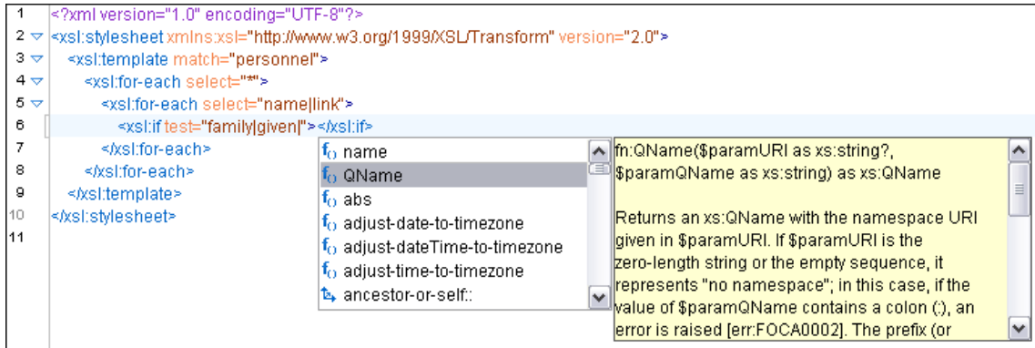
Figure 267. Content Completion in the @test Attribute
