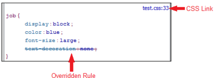
Figure 169. CSS Inspector View - Displaying Rules
