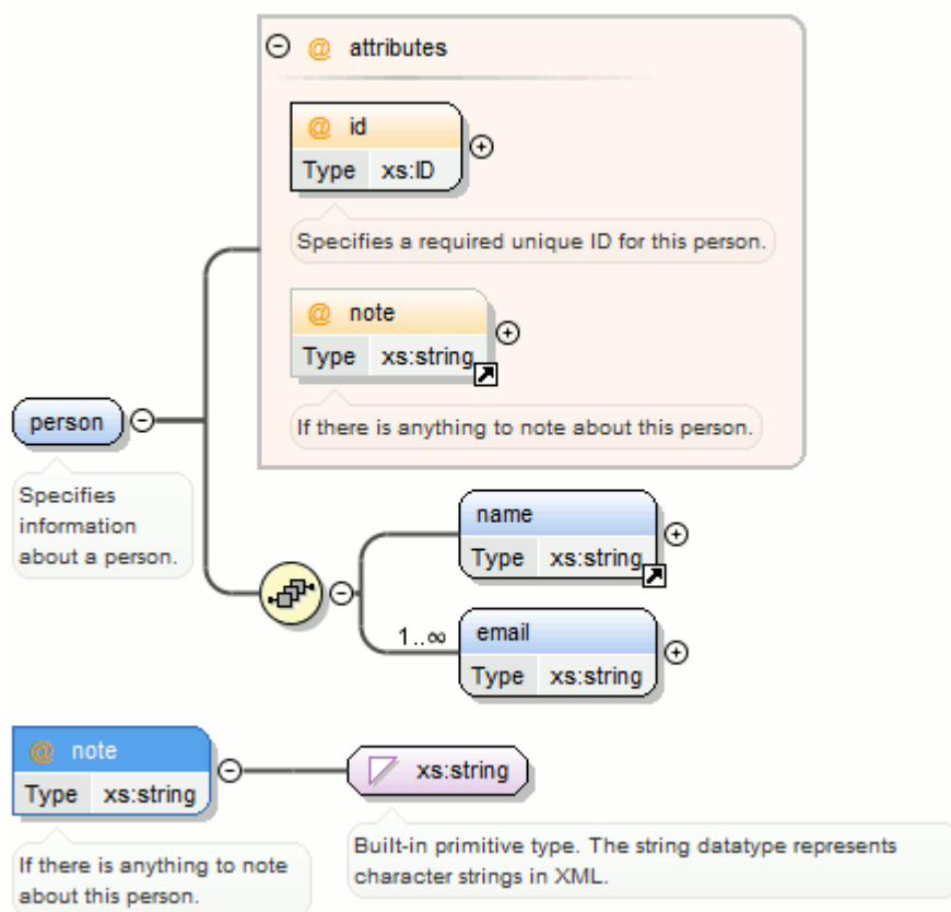
Figure 297. Extracting a Global Attribute on a @note Attribute
