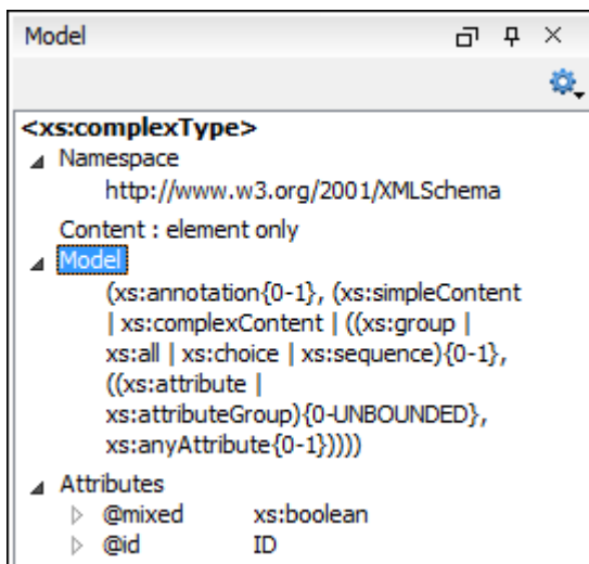
Figure 122. Element Structure Panel
