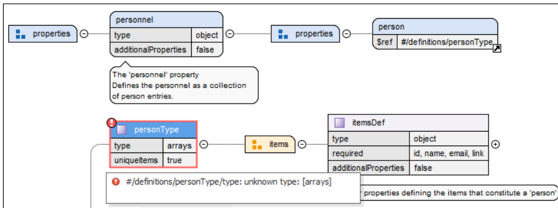
Figure 440. JSON Schema Design Mode Validation
