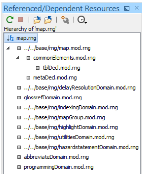
Figure 319. Referenced View
