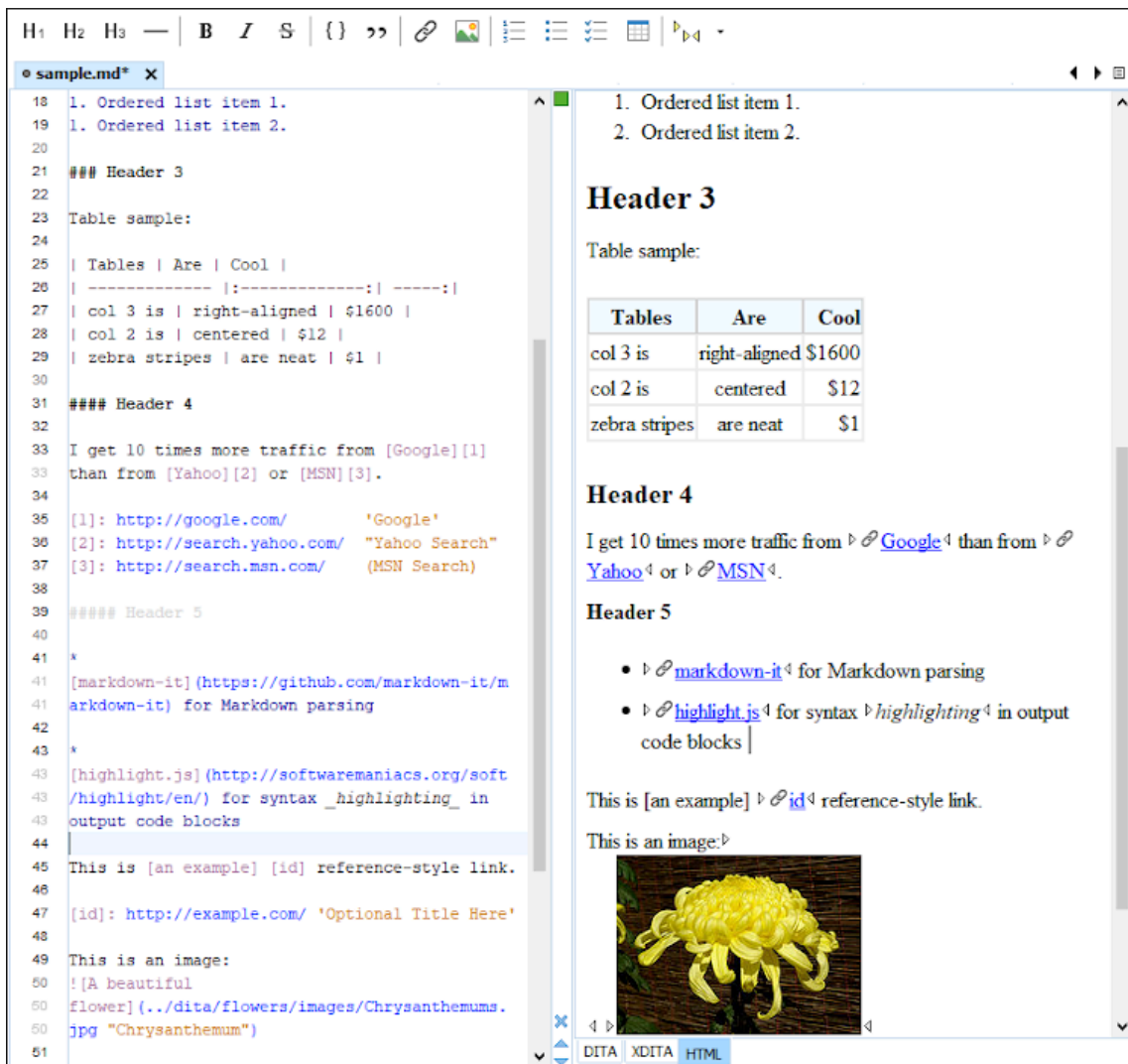
Figure 397. Markdown Editor
