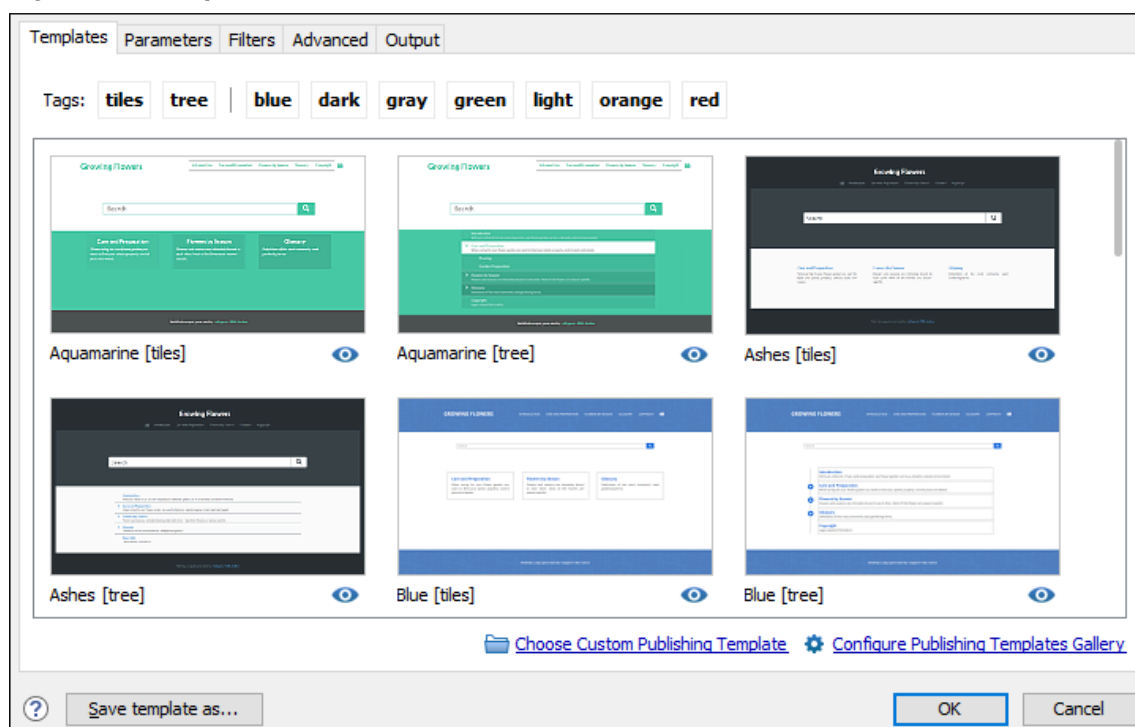
Figure 633. Templates Tab
