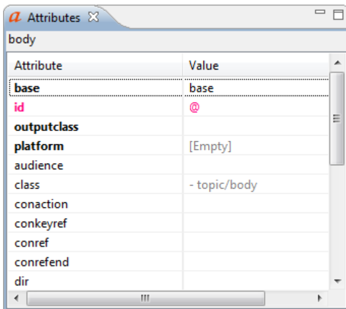
Figure 95. Attributes View
