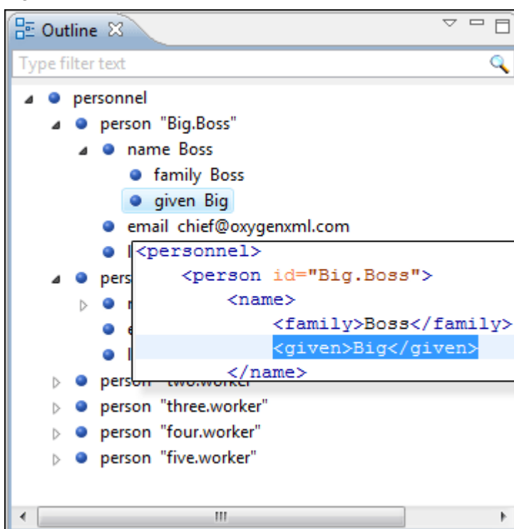
Figure 59. Outline View
