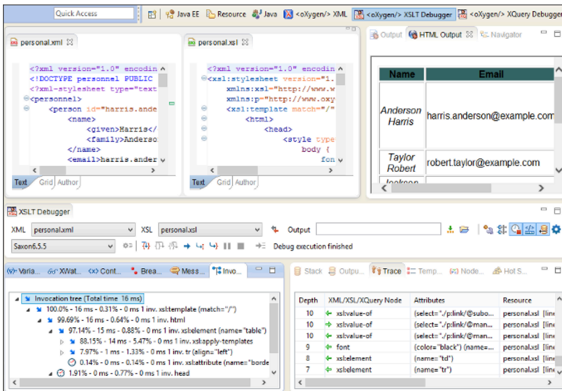
Figure 489. Debugger Interface
