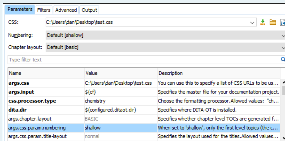
Figure 652. Promoted Parameters
