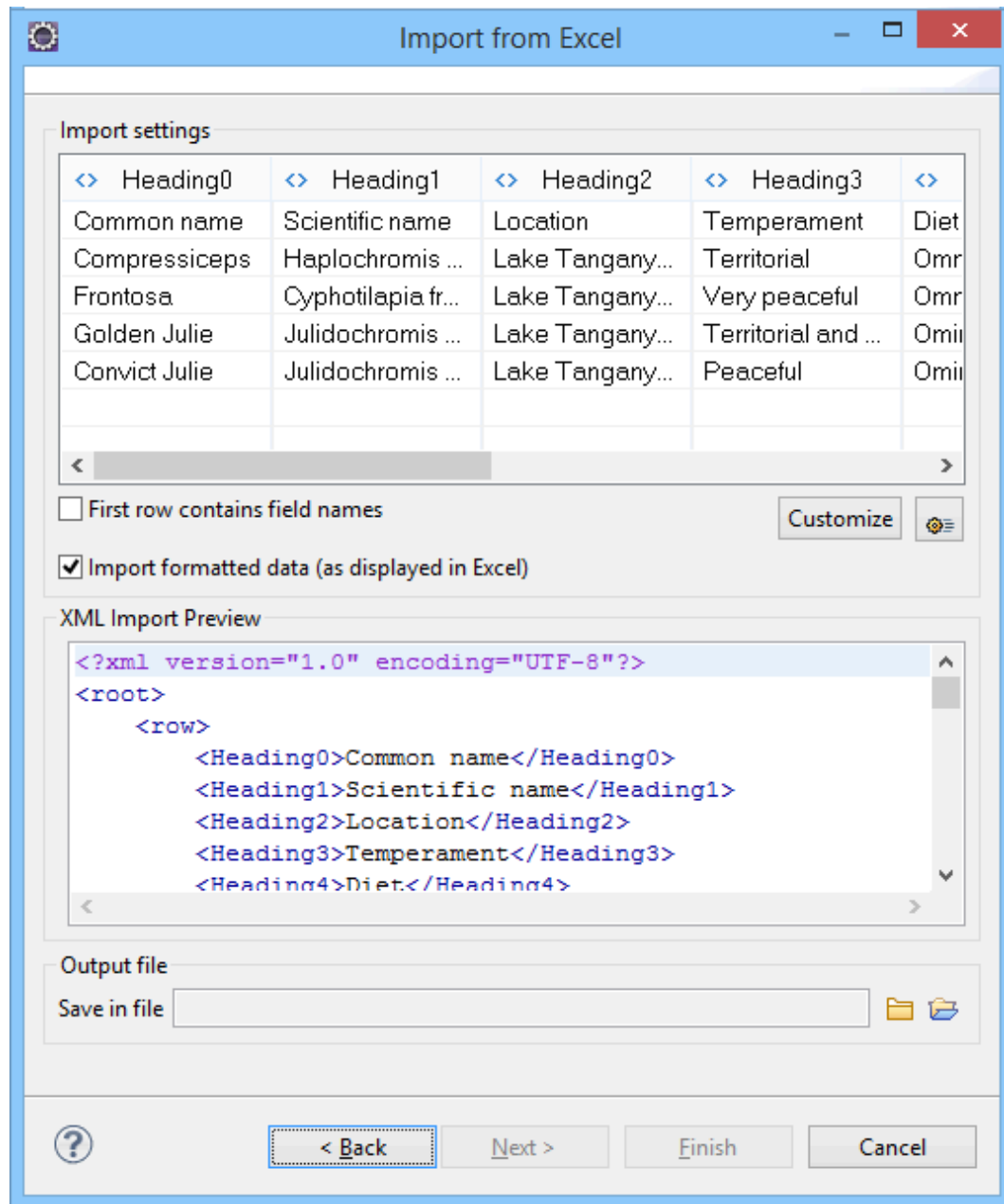
Figure 486. Import Wizard
