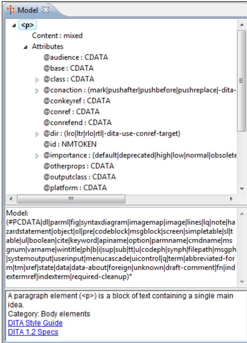
Figure 61. Model View
