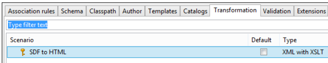
Figure 519. Transformation Tab
