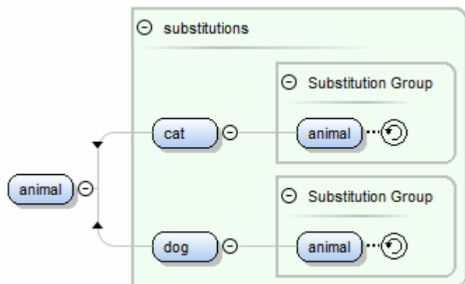
Figure 267. Substitutions Construct
