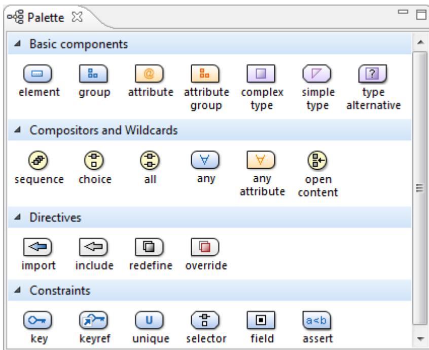
Figure 226. Palette View
