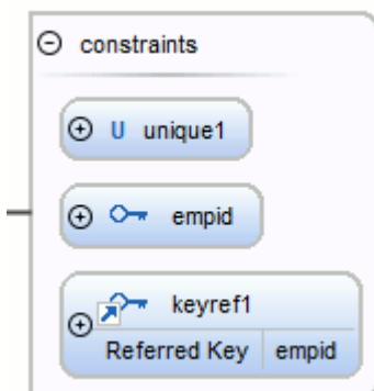
Figure 266. Constraints Construct
