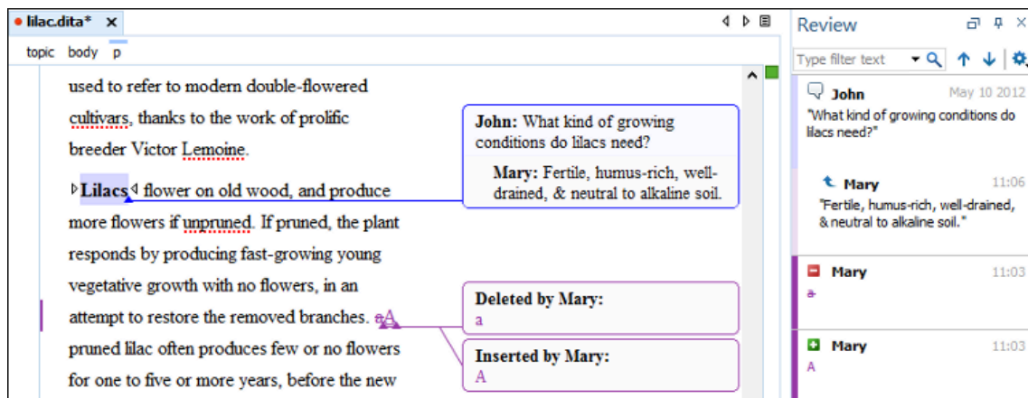
Figure 114. Review View
