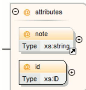
Figure 265. Attributes Construct
