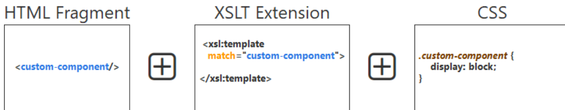
Figure 447. Custom Component
