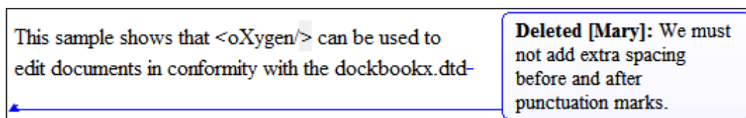
Figure 112. Deletion Callouts
