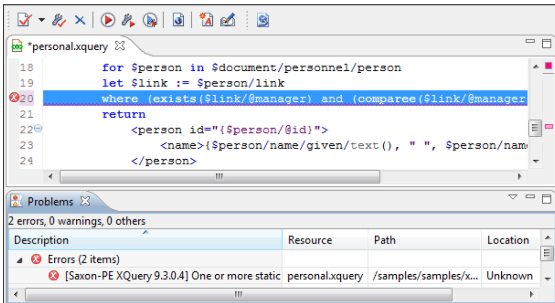
Figure 289. XQuery Validation
