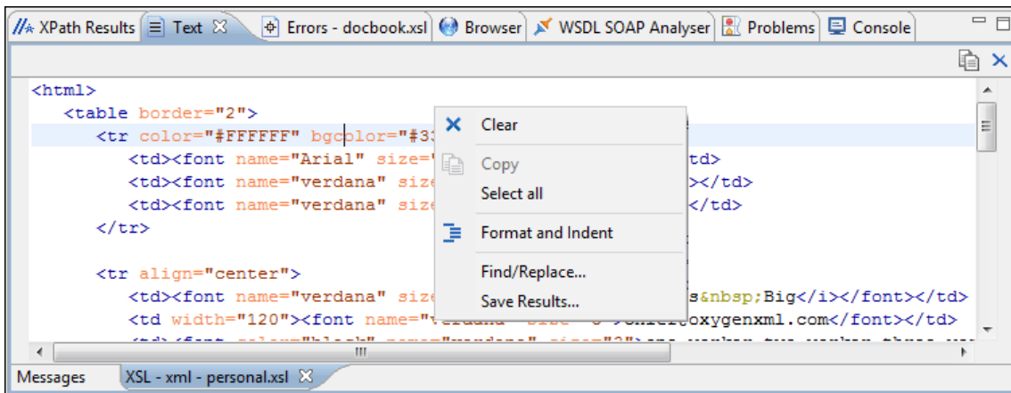
Figure 413. Text View
