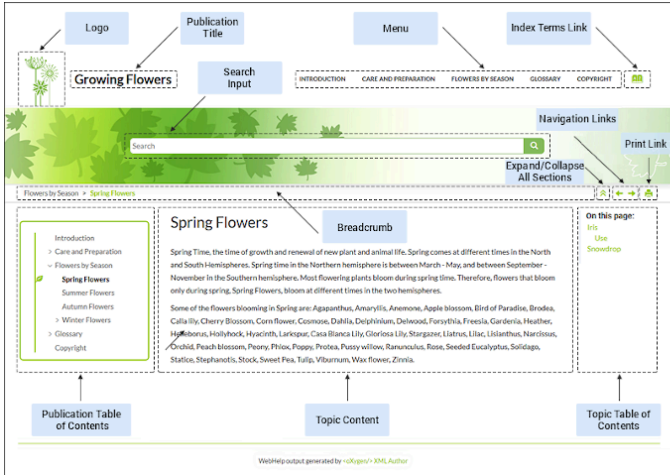
Figure 429. Topic Page
